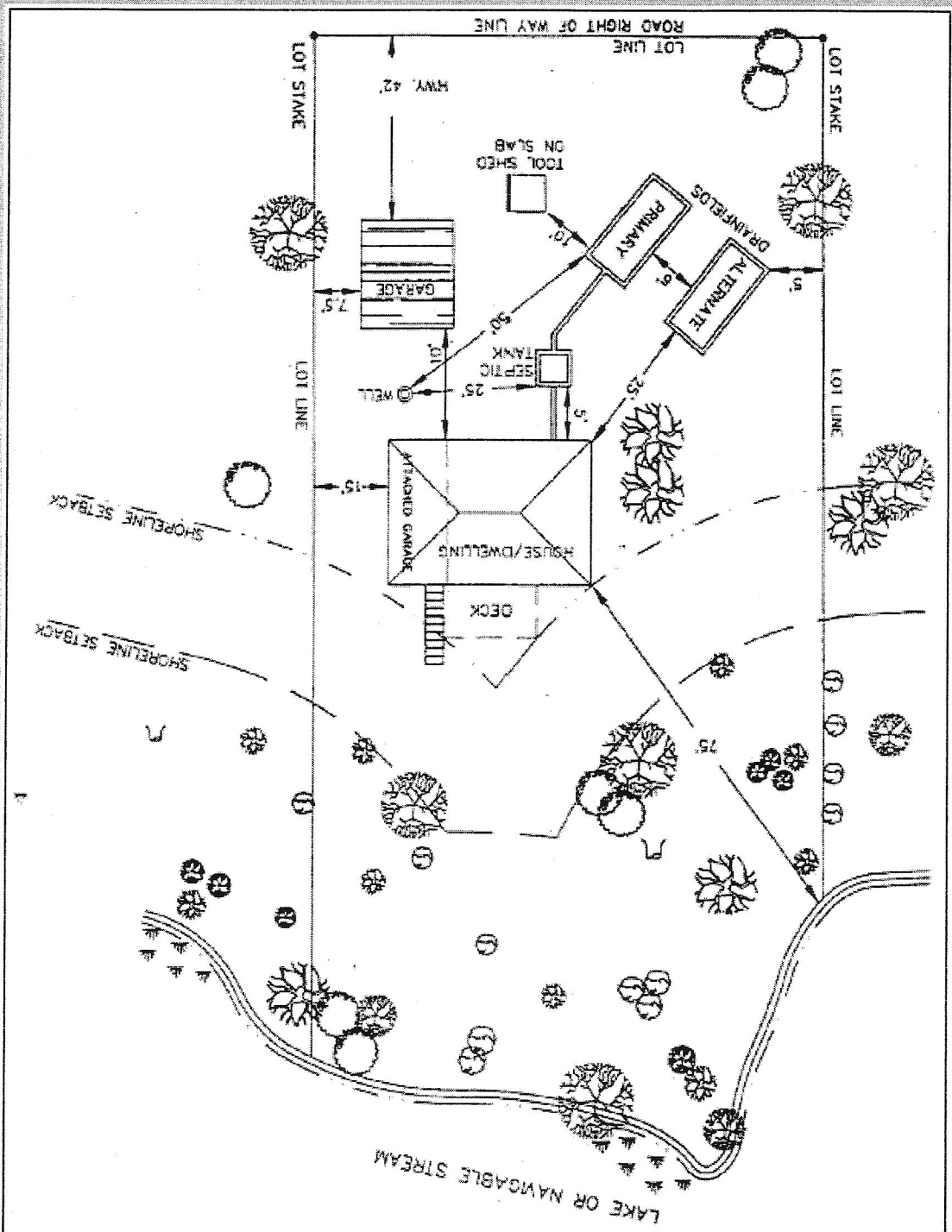
Example site plan provided by Langlade County, WI.
